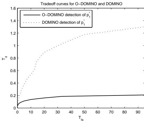
Fig. 9. Tradeoff curves for the original DOMINO algorithm with K = 3 , \gamma = 0.9 and different values of m vs. O-DOMINO with \gamma = 0.7 and different values of K
