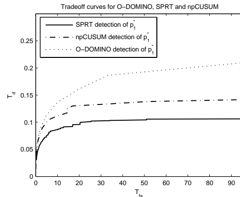
Fig. 11. Tradeoff curves for SPRT with b = 0.1 and different values of a vs. nonparametric CUSUM and O-DOMINO with \gamma = 0.7 and different values of K
