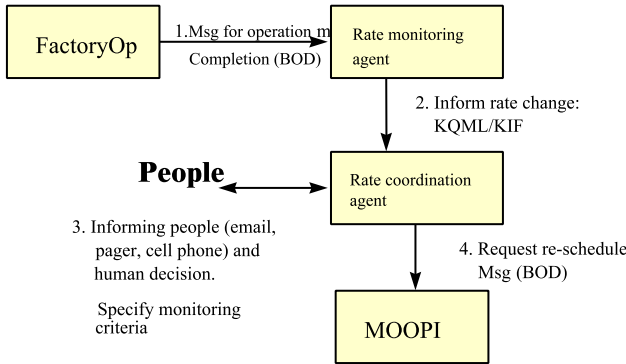
Figure 3. The “process rate change” scenario
