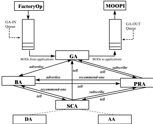
Figure 4. The agent system for “process rate change” scenario
