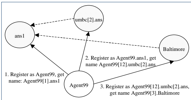
Figure 1. KNS Alias Network. The registrars of Agent99 coordinate to maintain the agent's distributed identity.
